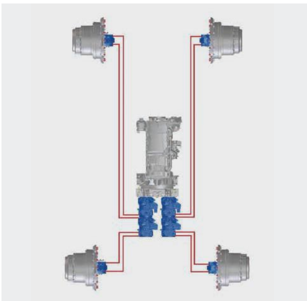
Quad-Pump-Drive (BC 573).
