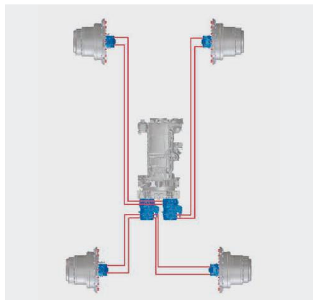
Dual-Pump-Drive (BC 463/BC 473).
